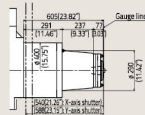
Spindle Shape and Dimensions
