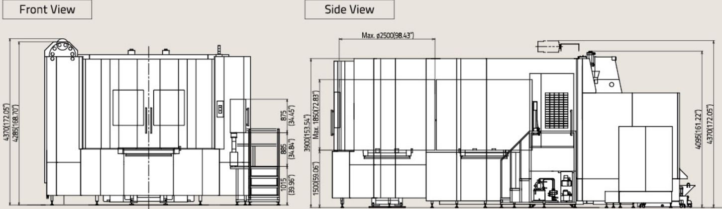
Floor Space Diagram
