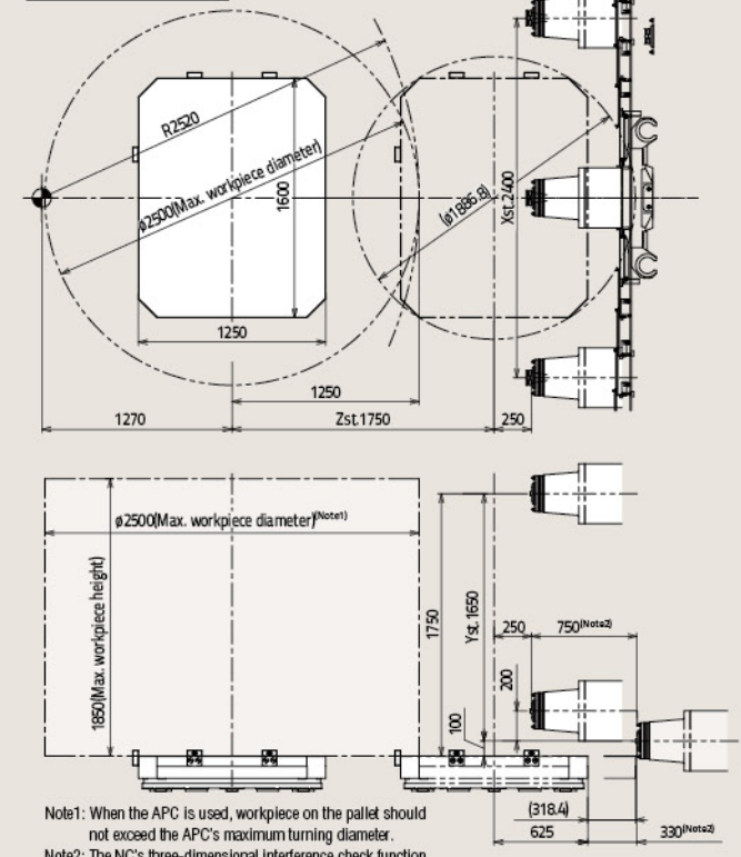
Stroke Diagram
