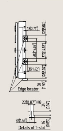
Pallet Dimensions
