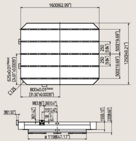
T-slot Specification [Option]
